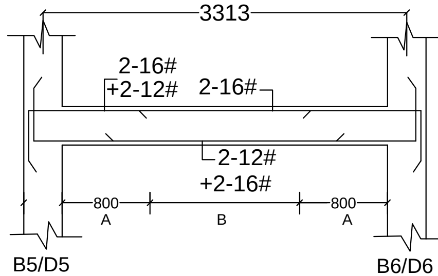
FL. BEAM -02 (BEAM SIZE-250X350)
