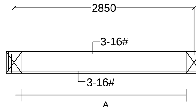
FL. BEAM -03 (BEAM SIZE-250X350)
